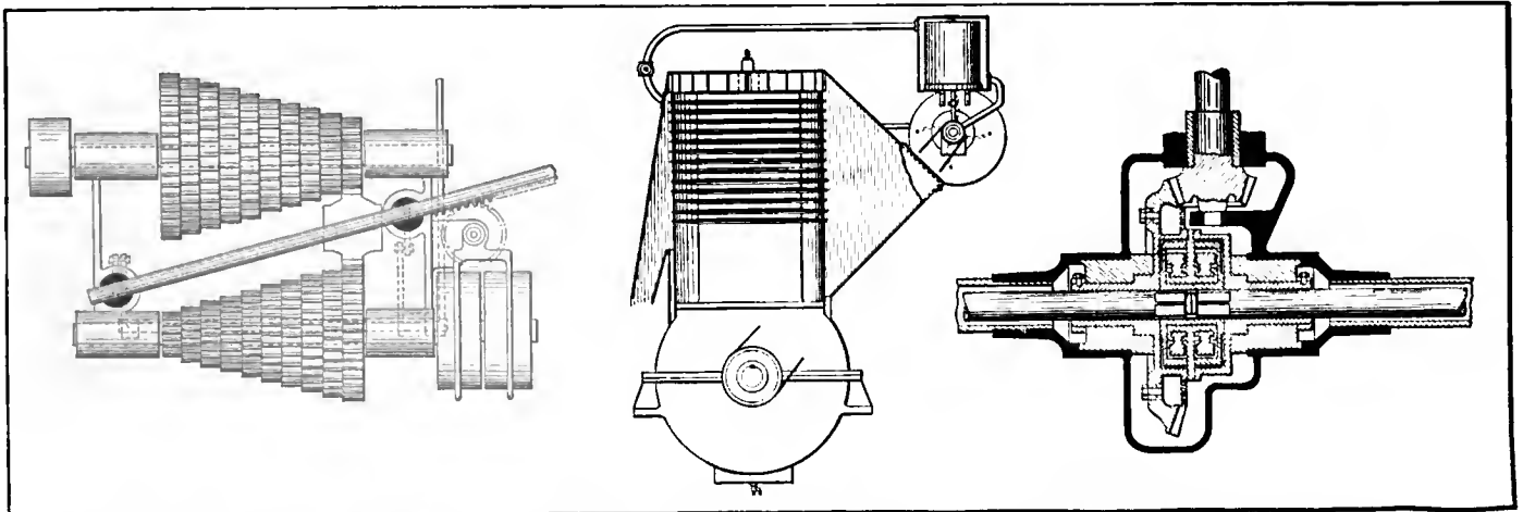
Fig. 3—Rogers compensating gearset
